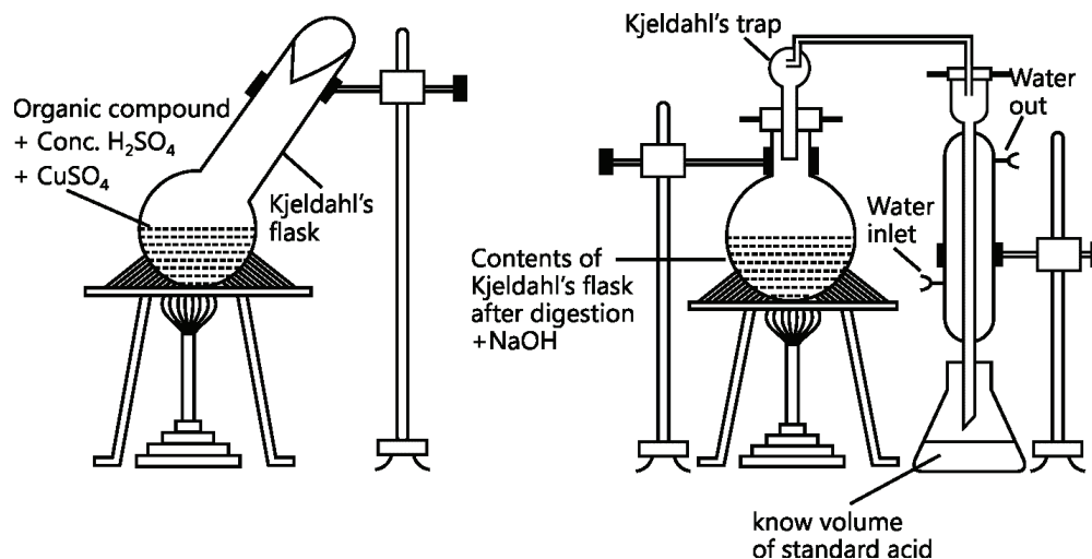
Figure 27.10: Kjeldahl's Method
