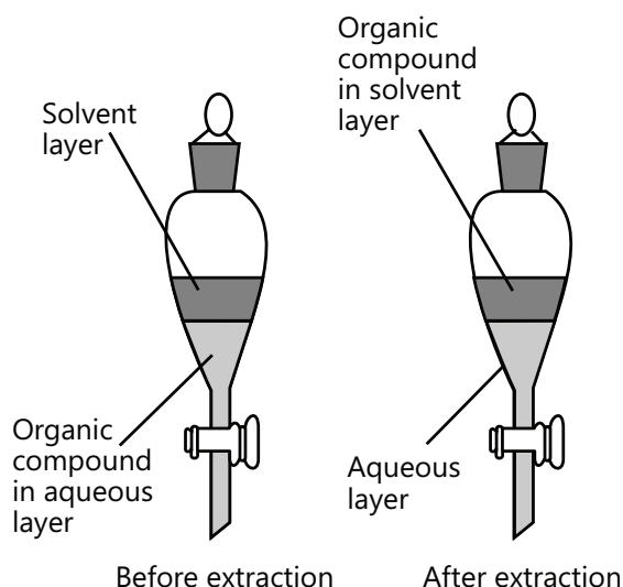
Figure 27.6: Separating Funnel
